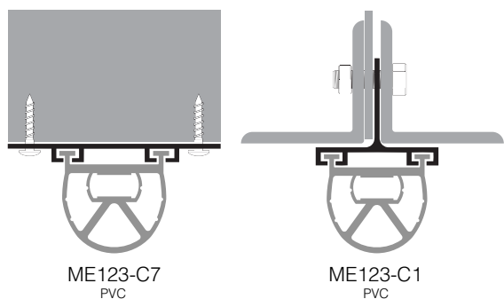
IMAGE 2: Mounting Channel Styles & Possible Hardware Placement
