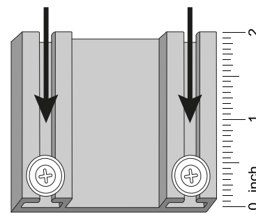
IMAGE 4: Installing the assembled edge (gates)
