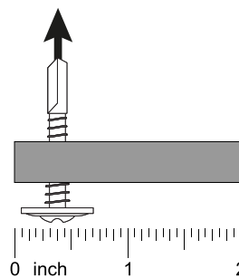
IMAGE 3: Installing a #8 x 1/2-in. lath screw
