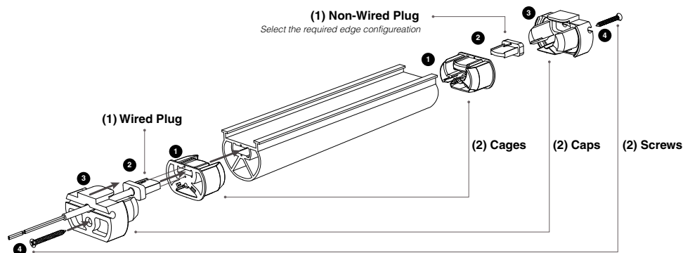
IMAGE 1: CPT215 Assembly
