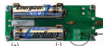
Fig. 2-6 WIRE CONNECTION TO TERMINAL BLOCK
